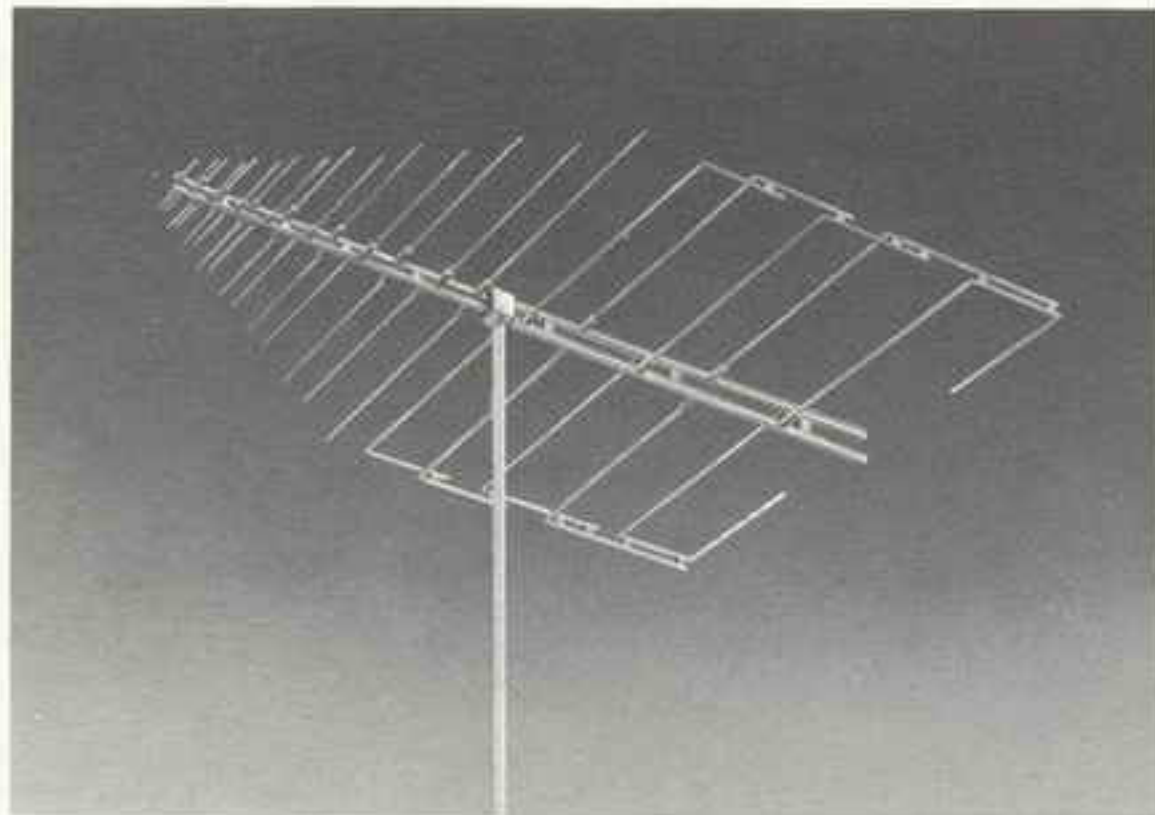
AR274-1 with AR272-1 mounted on top
