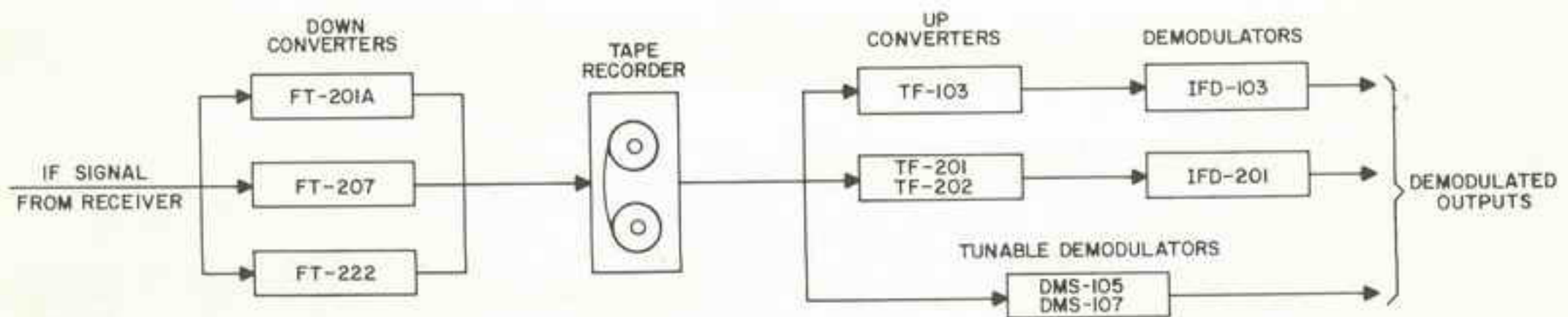
Block Diagram, Predetection Recording and Playback System
