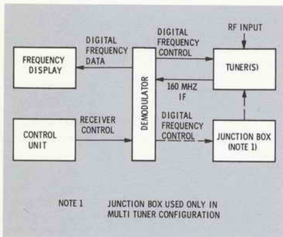
Basic Receiver
