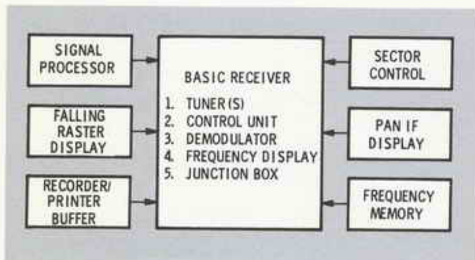
Basic Receiver and Selected Peripheral Equipment
