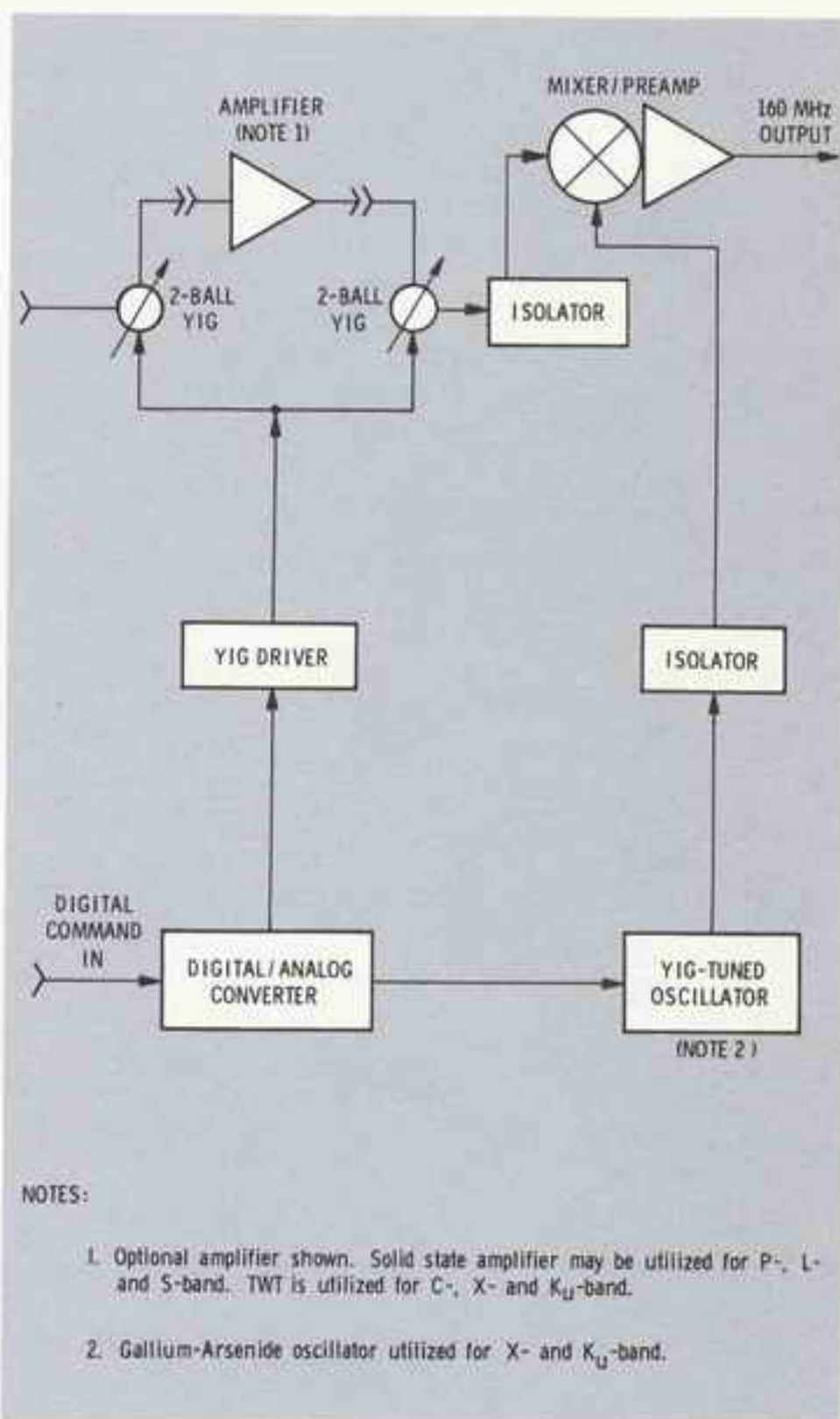
Tuner Block Diagram
